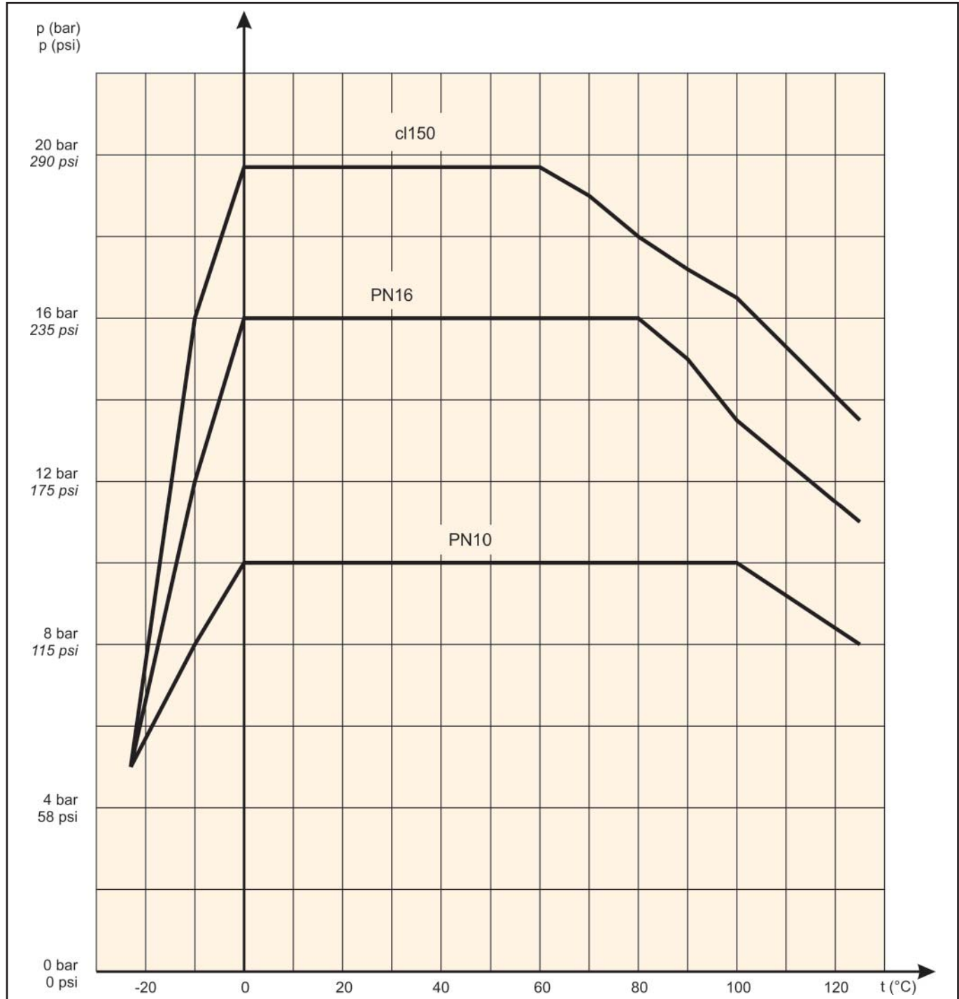
Fig. 4 - Pressure-Temperature diagram
