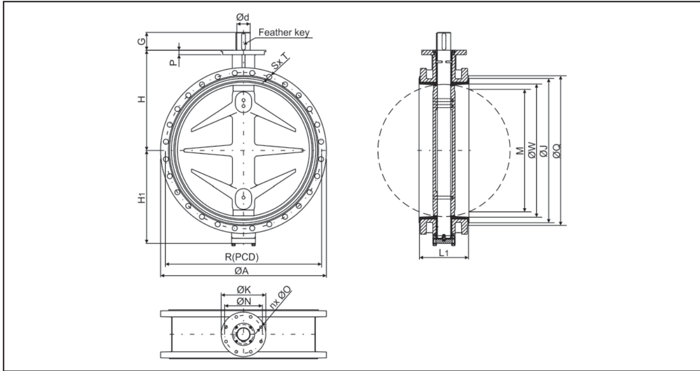
Fig. 14 - Double-flanged valve DN 700 to DN 1200 and NPS28 to NPS48
