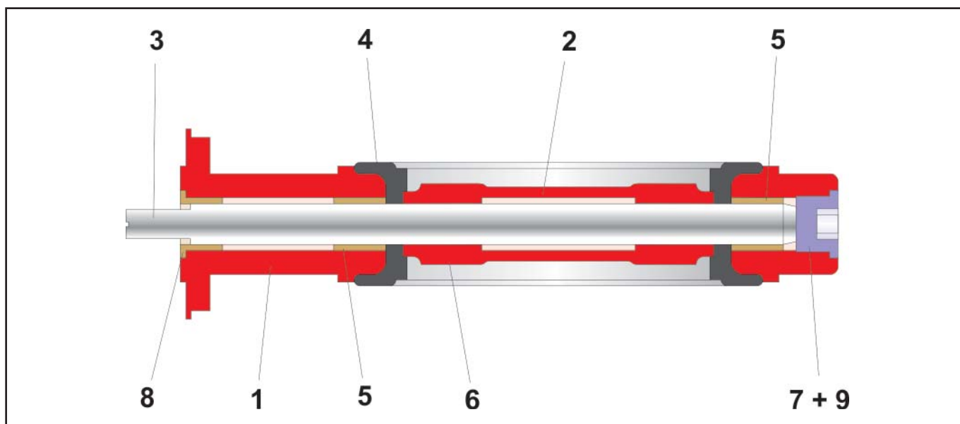
Fig. 3 - Cross-section of BR 11e Butterfly Valve
