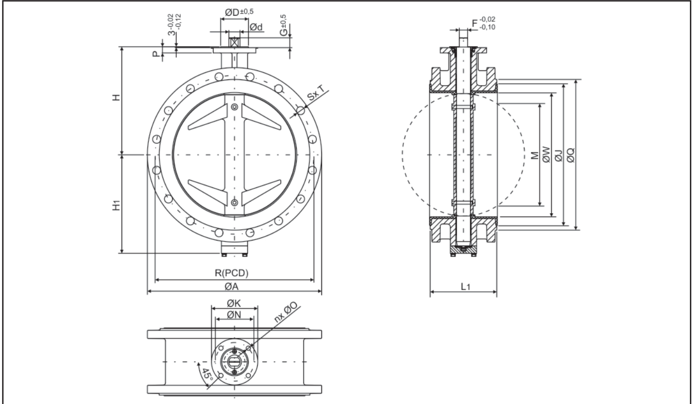
Fig. 13 - Double-flanged valve DN 250 to DN 600 and NPS10 to NPS24
