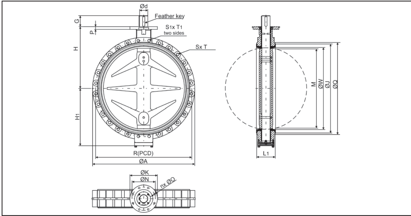
Fig. 8 - Lug-type valves DN 700 to DN 1200 and NPS28 to NPS48
