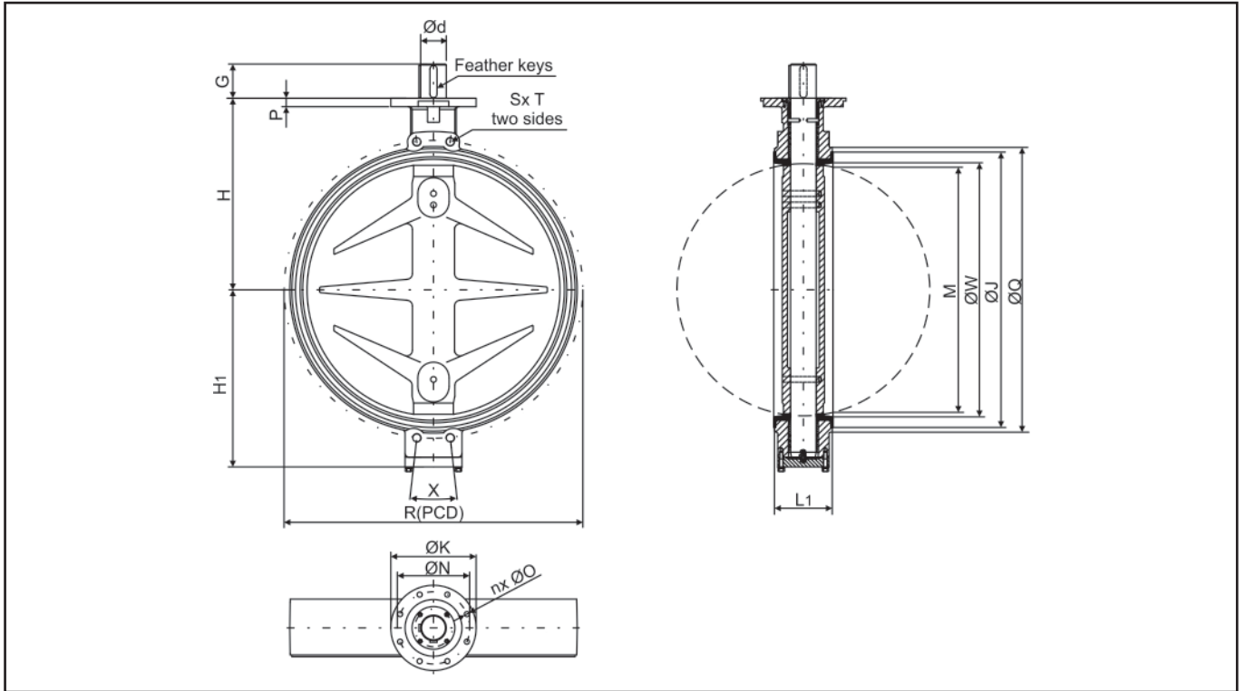
Fig. 11- Wafer-type valves DN 700 to DN 1200 and NPS28 to NPS48
