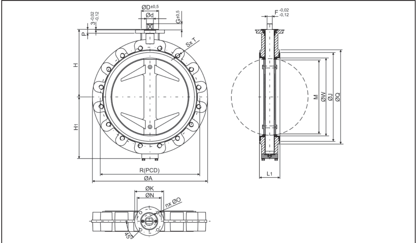
Fig. 7 - Lug-type valves DN 250 to DN 600 and NPS10 to NPS24
