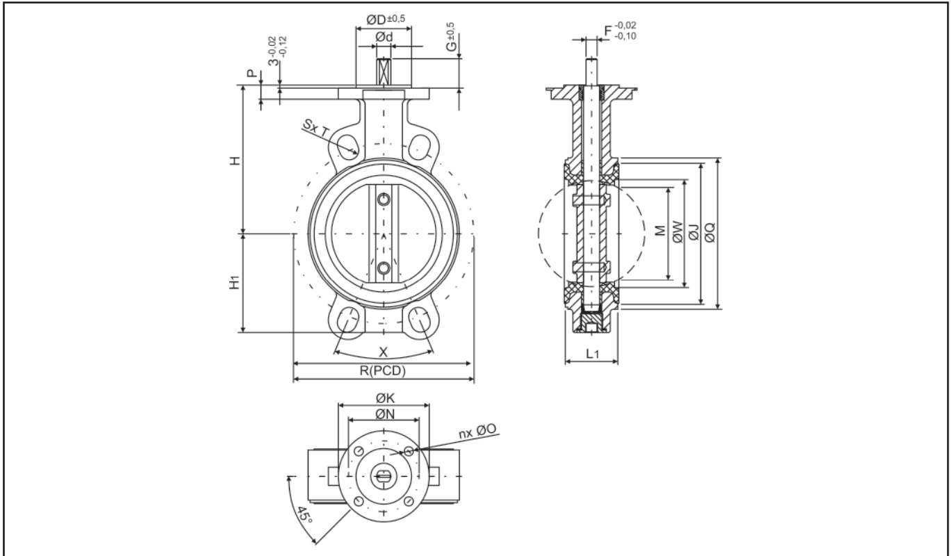
Fig. 9 - Wafer-type valves DN 40 to DN 200 and NPS1½ to NPS8
