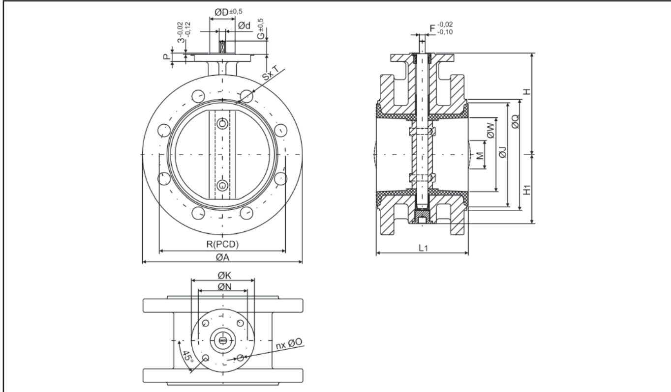
Fig. 12 - Double-flanged valve DN 50 to DN 200 and NPS2 to NPS8
