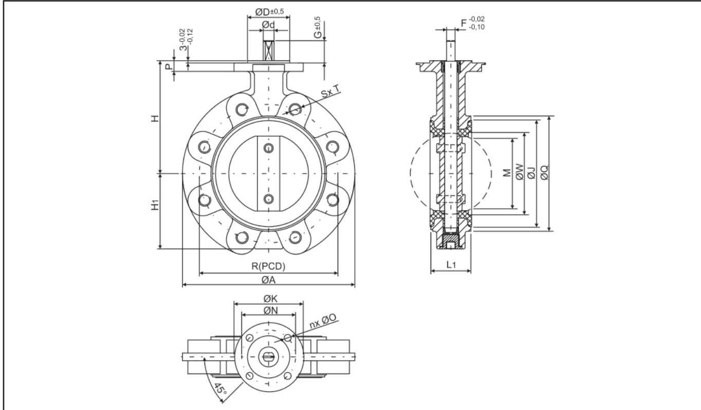
Fig. 6 - Lug-type valves DN 40 to DN 200 and NPS1½ to NPS8
