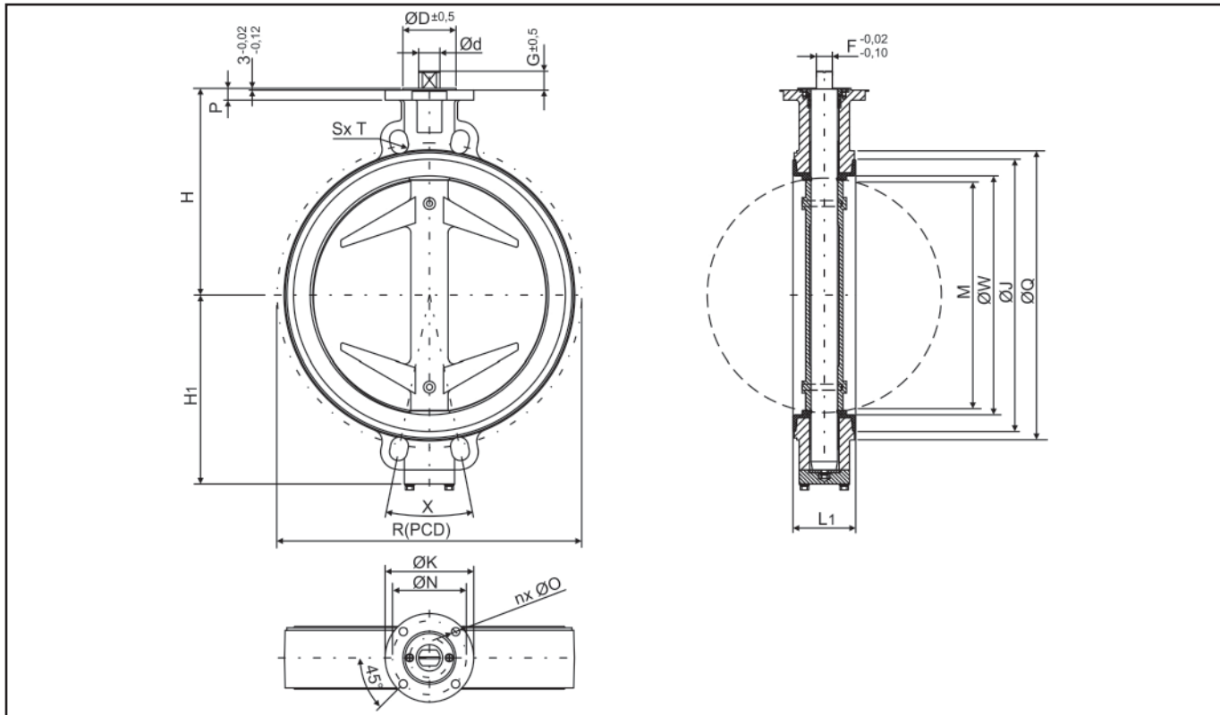
Fig. 10 - Wafer-type valves DN 250 to DN 600 and NPS10 to NPS24
